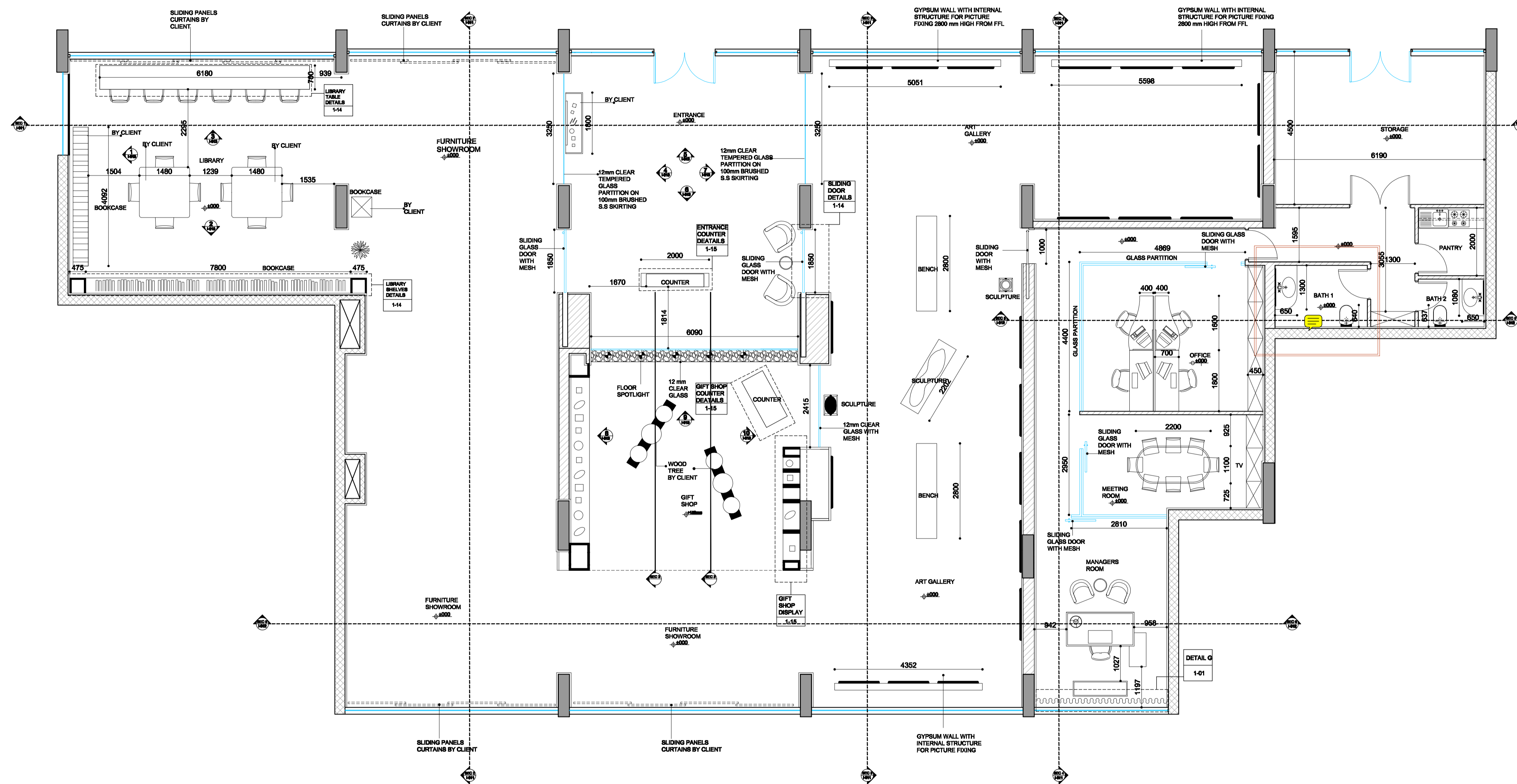
FURNITURE LAYOUT I-01 SCALE 1:75
